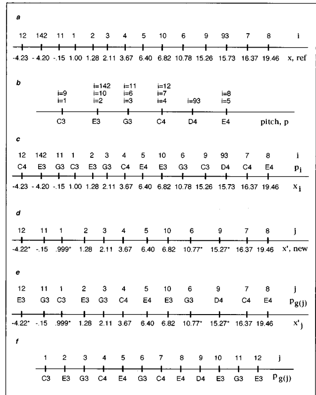
FIG. 1. Generating the first 12 pitches of Variation 1 [Fig. 2(b)]. (a) The first 12 x -components \{x_i\} , i=1, \dots, 12 , of the reference trajectory starting from the IC (1,1,1) are marked below the x axis (not drawn to scale). Two more x -components, that will later prove significant, are indicated: x_{93}=15.73 and x_{142}=-4.20 . (b) The first 12 pitches of the Bach Prelude are marked below the pitch axis. The order in which they are heard is given by the index i=1, \dots, 12 . The 93rd and 142nd pitches of the original Bach are also given. (c) Parts (a) and (b) combine to give an explicit pairing. (d) The first 12 x' -components of the new trajectory starting from the IC (0.999, 1, 1) are marked below the x' axis (not drawn to scale). Their sequential order is indicated by the index j=1, \dots, 12 . Those x'_j \neq x_i , i=j , are starred. (e) For each x -component x'_j , apply the chaotic mapping. All pitches remain unchanged from the original until the ninth pitch. Because x'_9 = 15.27 \leq x_{93} = 15.73 , x'_9 adopts the pitch D4 that was initially paired with x_{93} . The next two pitches of Variation 1 replicate the original Bach, but the twelfth pitch, E3, arises because x'_{12} \leq x_{142} = -4.20 \rightarrow E3 . (f) The variation is heard by playing back p_{g(j)} for j=1, \dots, N , where N=176 , the number of pitches in the first 11 measures of the Bach.
