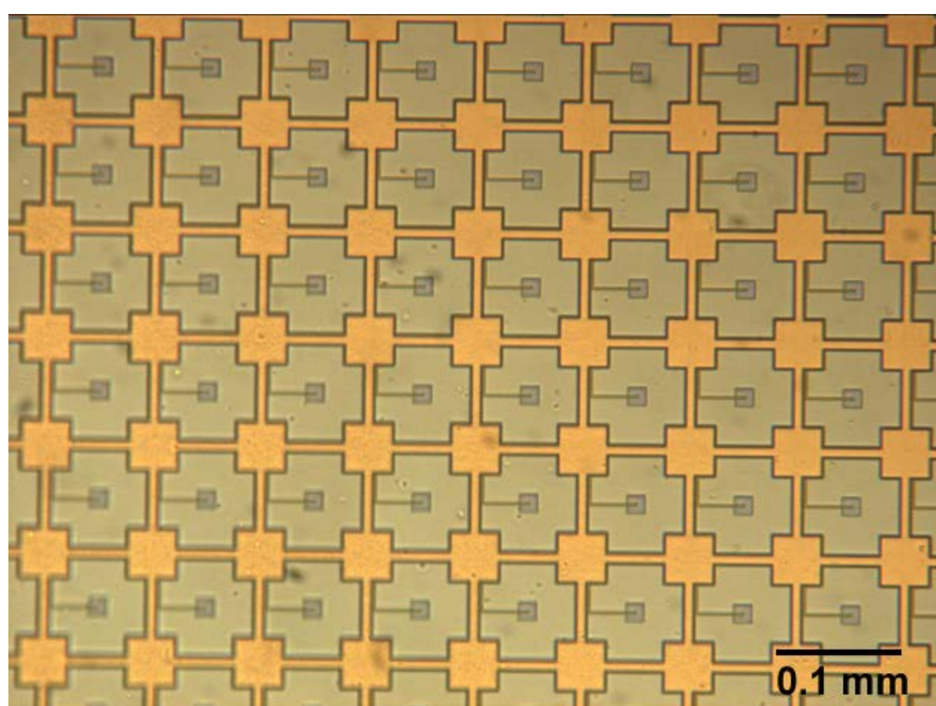
Optical micrograph of a photo detector array inside an Agilent optical mouse chip
