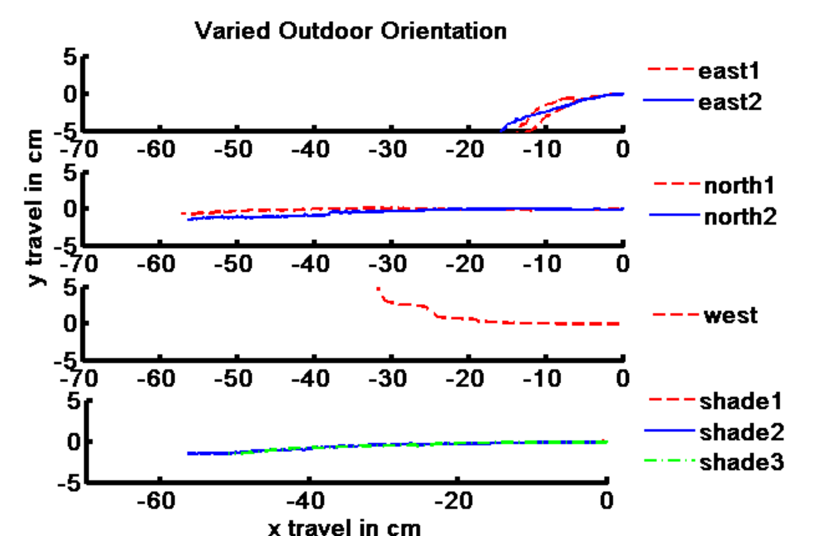
Optical Mouse Results using the ER-1 platform with different lighting conditions
