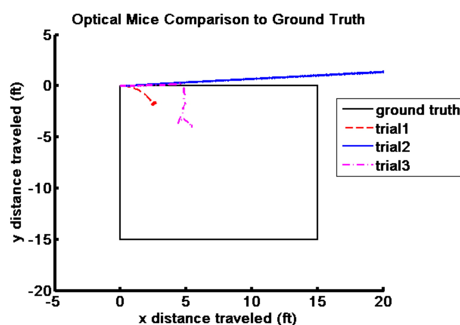
Optical Mouse Results from three box tests on Integrated Platform
