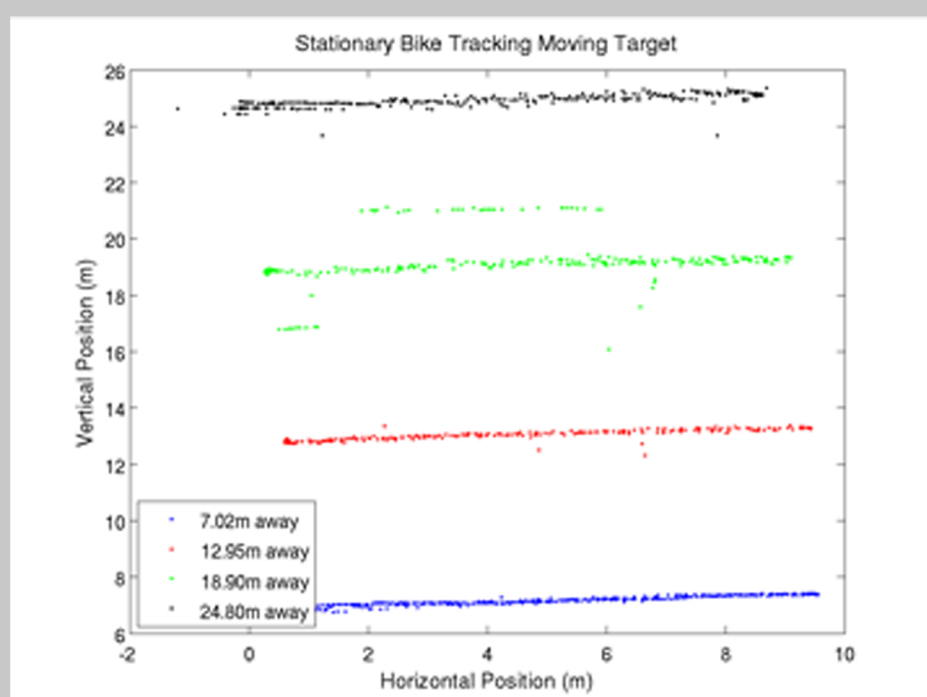
Figure 2: In this test, we tracked a target moving perpendicular to the stationary bike's line of sight. The colored lines represent tracking the target at different distances from the bike. Generally, deviations from the line along which the target was moving were small and on the order of 10cm. The larger errors were likely caused by the errors in the LIDAR, which has a tendency to produce erroneous results.
