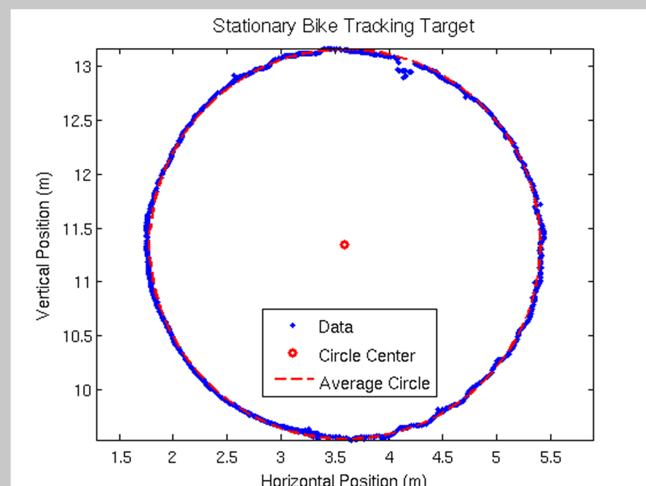
Figure 1: This image shows a circle we traced out with the target while keeping the bike stationary. Overall, it is very circular (especially compared to the red outline) with small deviations that are mainly caused by the difficulty in keeping the target perfectly aligned while walking about the circle. This test indicates that we can achieve good precision with our system.
